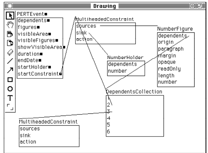
Figure 5 - The Diagramming Inspector
